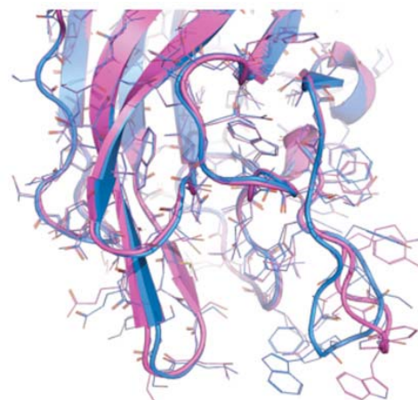
Fig. (5). The two known conformations of the discoidin C2 domain of coagulation factor Va, open (magenta) and closed (blue).
