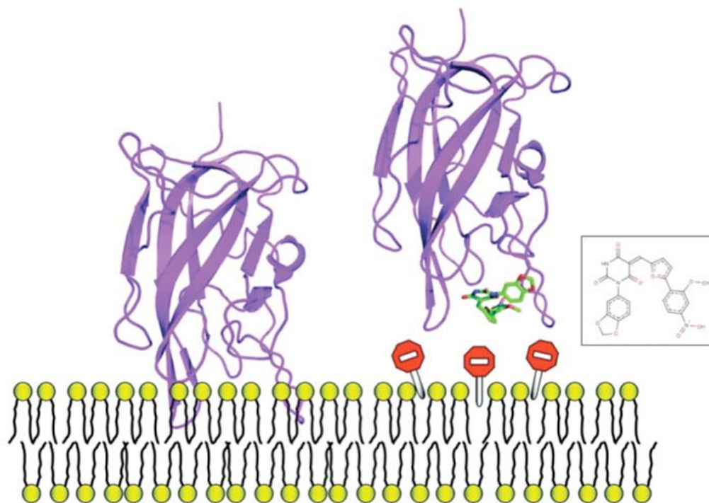
Fig. (6). Example of one small molecule identified in the FV-membrane study that impedes protein-membrane interaction, it can be used as a mechanistic probe to investigate this molecular event or, could be used as a starting point to develop anticoagulant molecules.
