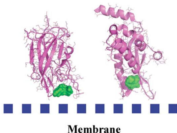
Fig. (4). Detected cavities (green) with the computer tool PASS [66], on Factor Va (left) and the PX-domain (right).
