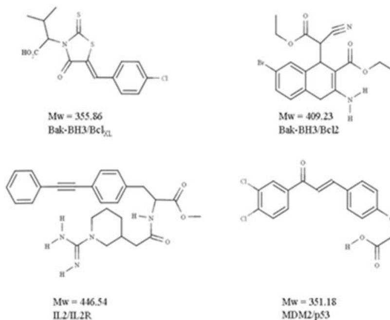
Fig. (3). Examples of “drug-like” protein-protein antagonists.
