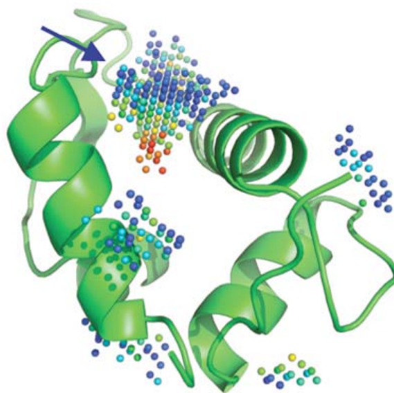
Fig. (2). Five cavities detected by PocketPicker [37] on MDM2. The predicted deepest and largest pocket (blue arrow) is indeed the key binding site for p53 and small molecules impeding p53 binding. Red spheres represent regions that are more buried in the protein interior as opposed to blue spheres, that become fully solvent exposed when the color shift to navy blue.
